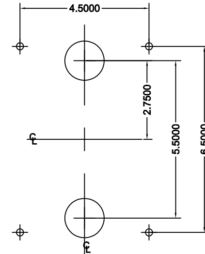
BACKPLATE CUT-OUT & MTG. DETAIL
